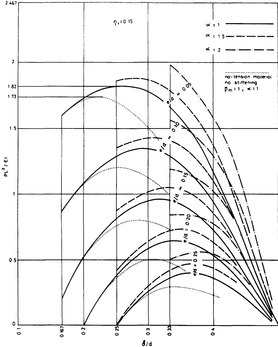
Fig. 3. Load vs deflection for various eccentricities and \alpha 's.
